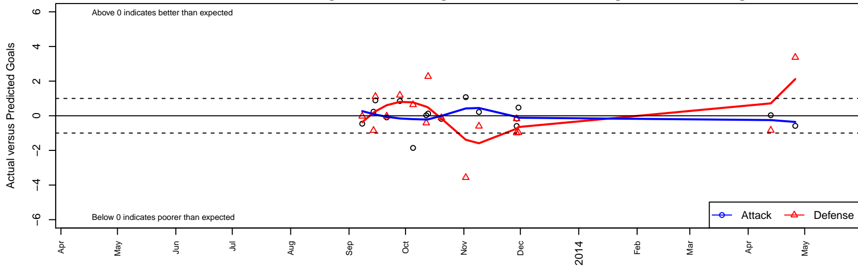
Cypress FC Black B98 Dots are actual minus expected GF (blue circles) and GA (red triangles). Blue line is smoothed change in attack strength. Red is smoothed change in defense strength.
